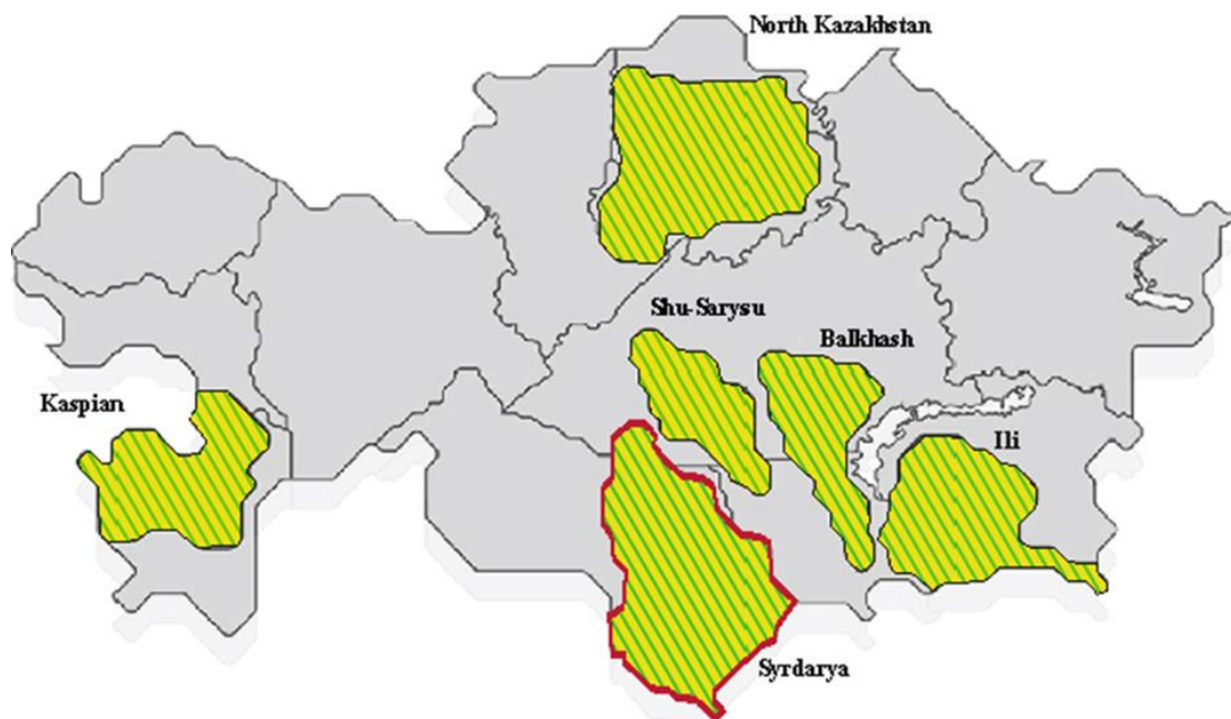
Figure 1. Uranium provinces of Kazakhstan, indicating the distribution of uranium reserves: Syrdarya (10.2%); North Kazakhstan (13.1%); Shu—Sarysu (66.8%); Ili (6.1%); Caspian (3.1%); Pribalkhashskaya (0.7%) [7].
